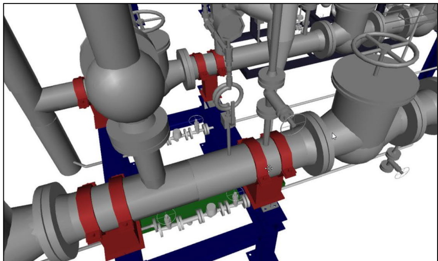
Pictures from a Raw Steam installation on a Pharmaceutical Factory – with Main Steam, 2 off pressure reduction stations, re-evaporation of condensate, condensate collection tank and condensate pumps.
