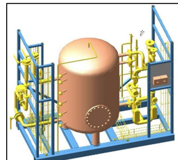
Pictures from a various installation in Denmark, Turkey, and the United Kingdom of Steam & Heating, Condensate, Steam Generation and Hot Tap Water Production.
