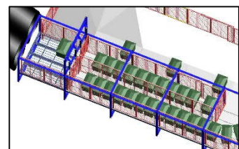
Pictures for design of a Special Waste Transport System for Waste Incineration Plant in Denmark.
