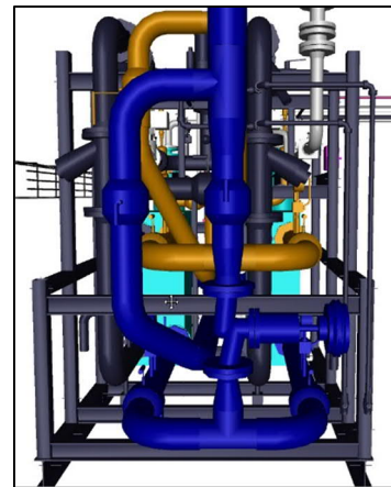
Pictures from a Utility Installation in relation with a pharmaceutical plant (DK).
