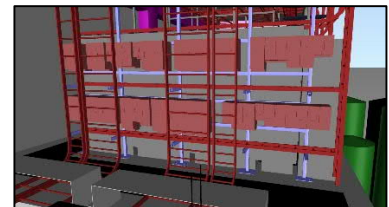
Example Electrical Room Layout with PDBs, MCCs and Free standing VSDs.
